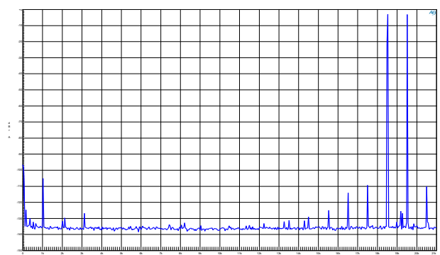
IMD spectrum at 18.5kHz + 19.5kHz, P_R/2 in 4Ω (blue).
