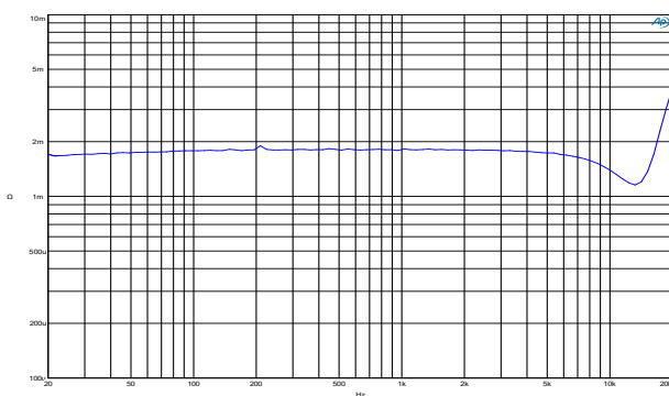
Output impedance
