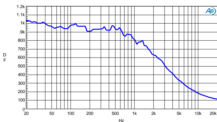
Figure 25: Damping factor in 8 \Omega BTL
