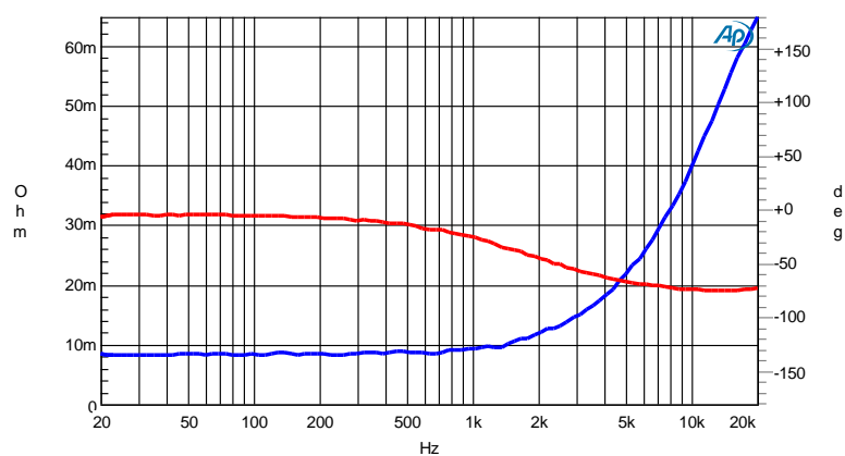
Figure 24: Output Impedance BTL (Blue), and Phase (Red)
