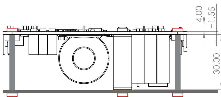
Figure 7: ICEpower400A2 Side view Heatsink mounting example with 30 mm spacers.
